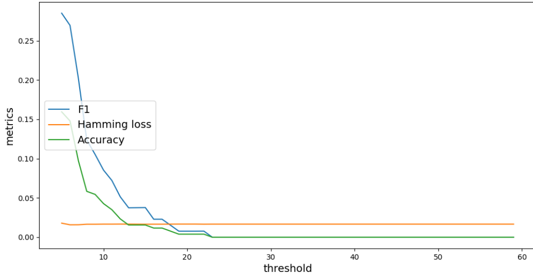
Classifier Chain Model
